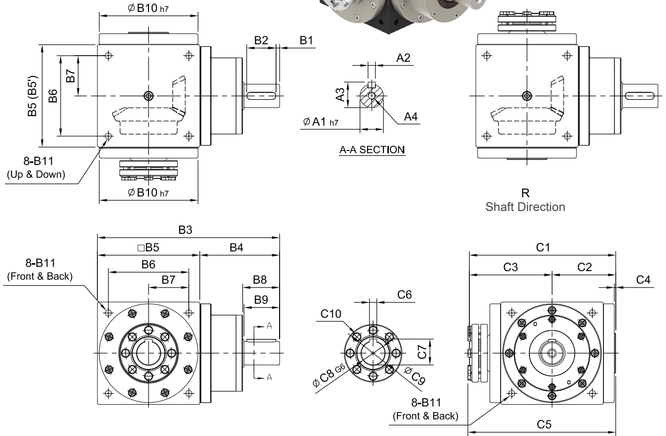
Single Input Shaft - Single Clamping
